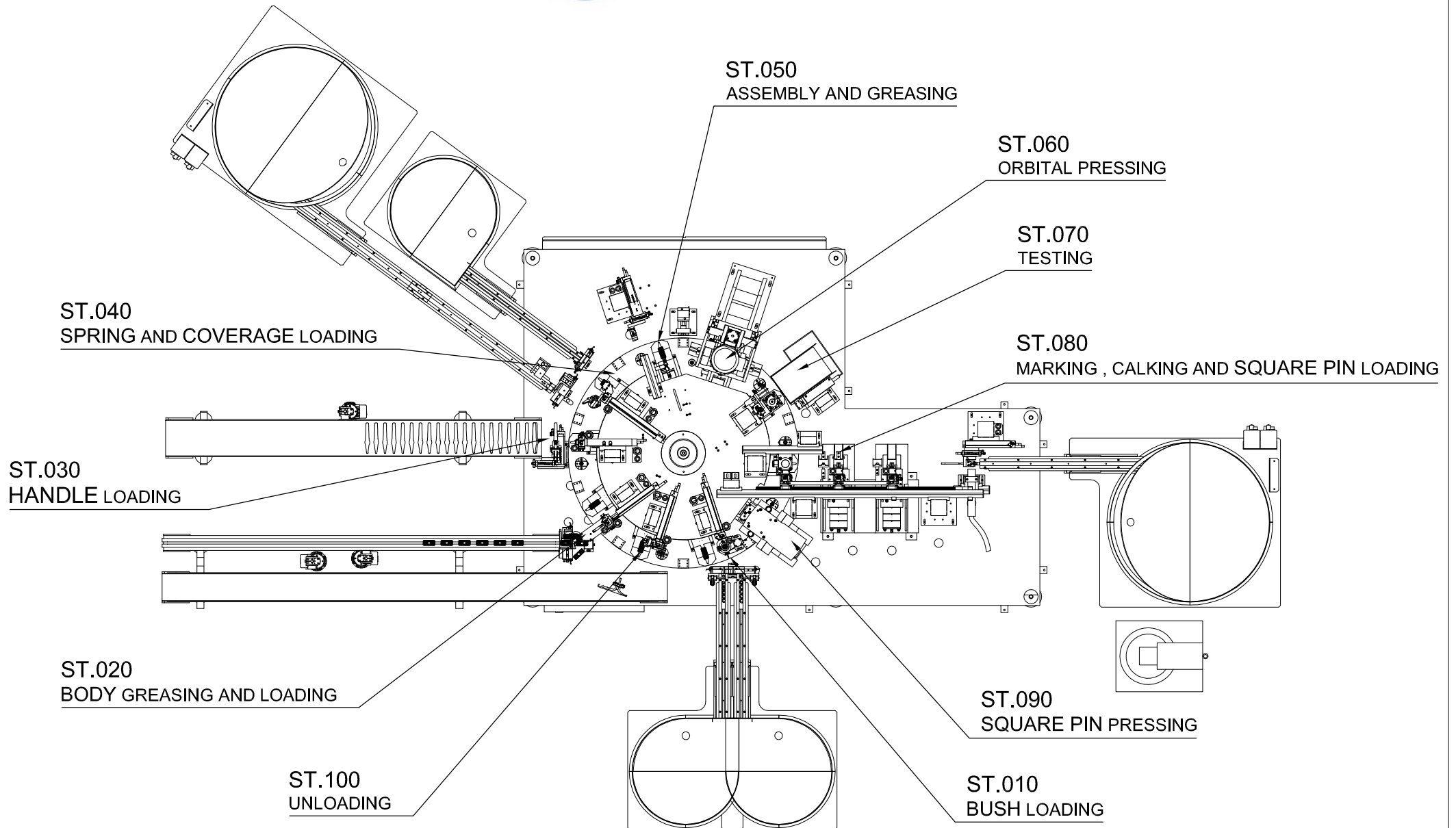
ASSEMBLING AND TESTING MACHINE FOR WINDOWS HANDLES
